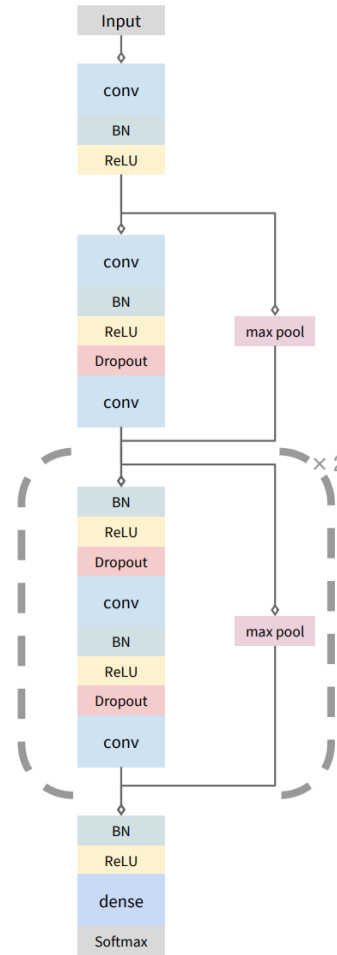
Figure 2: Architecture of the 1-D convolutional ResNet.
